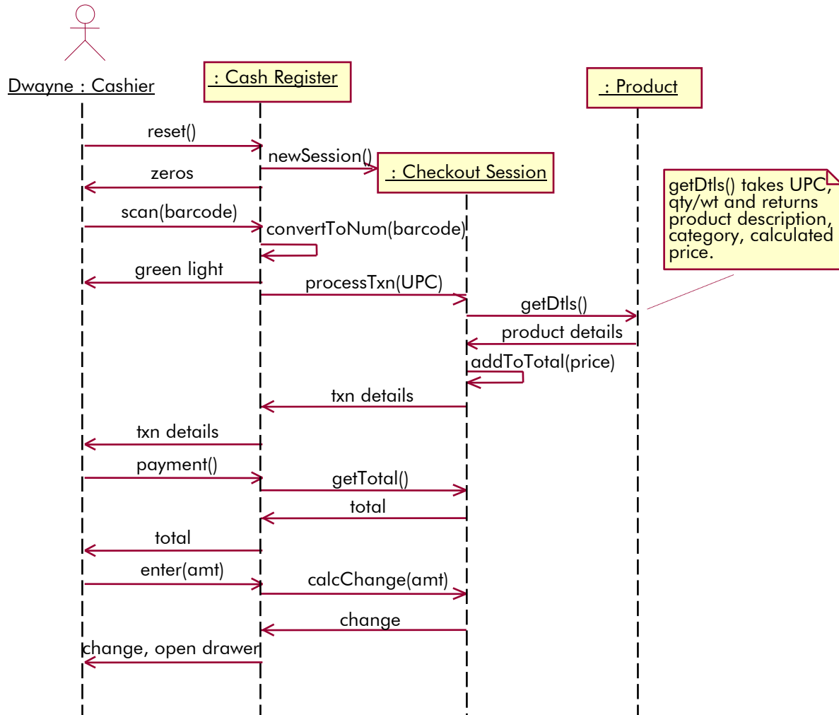
Sequence Diagram 1: A checkout session consisting of one successfully scanned item
