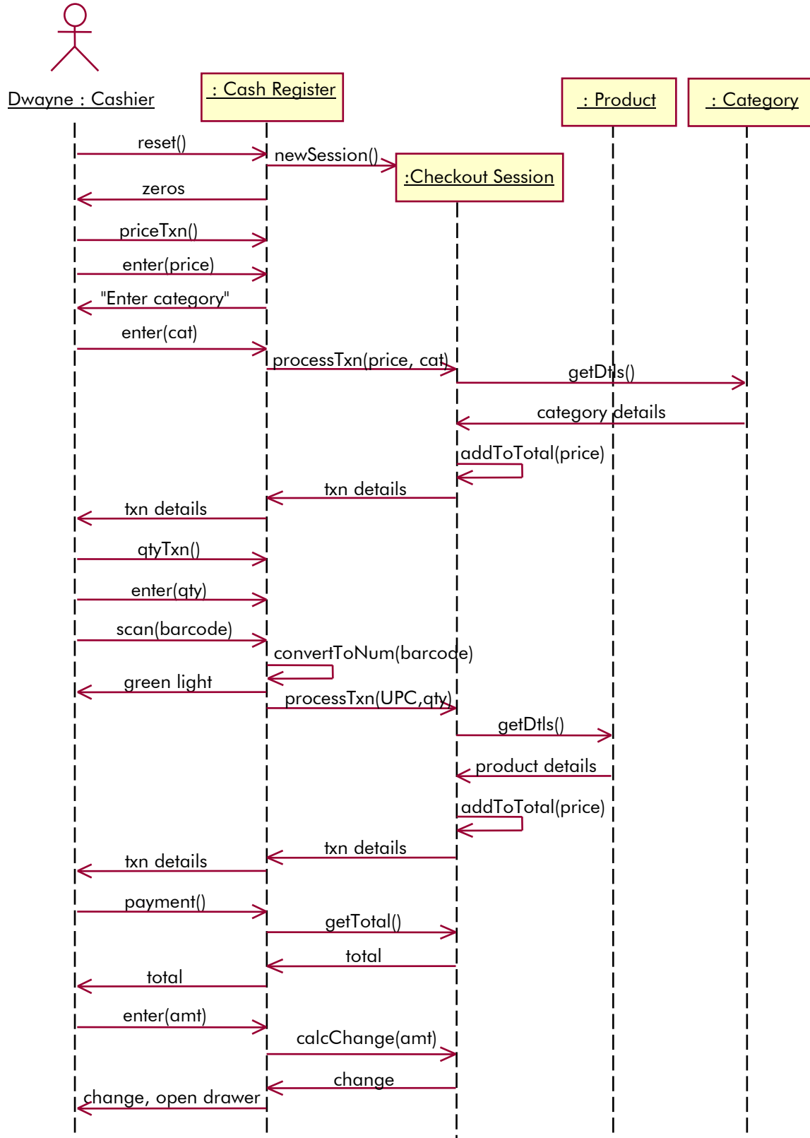
Sequence Diagram 4: A checkout session consisting of a price entry transaction and a number of identical items having a readable bar code
